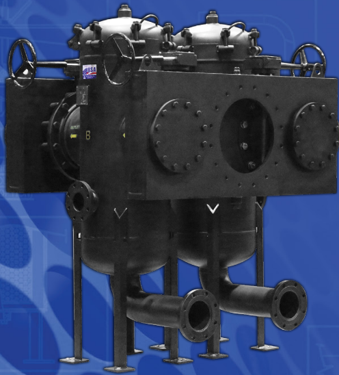
16" Fabricated Box Duplex Strainer with hinged cover
