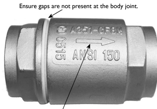
Flow arrow must be pointed in the direction of the flow.
